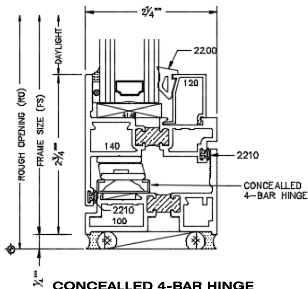
CONCEALED 4-BAR HINGE Casement / Awning / Hopper
