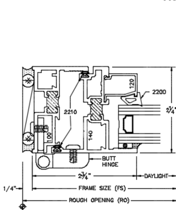
BUTT HINGE Casement
