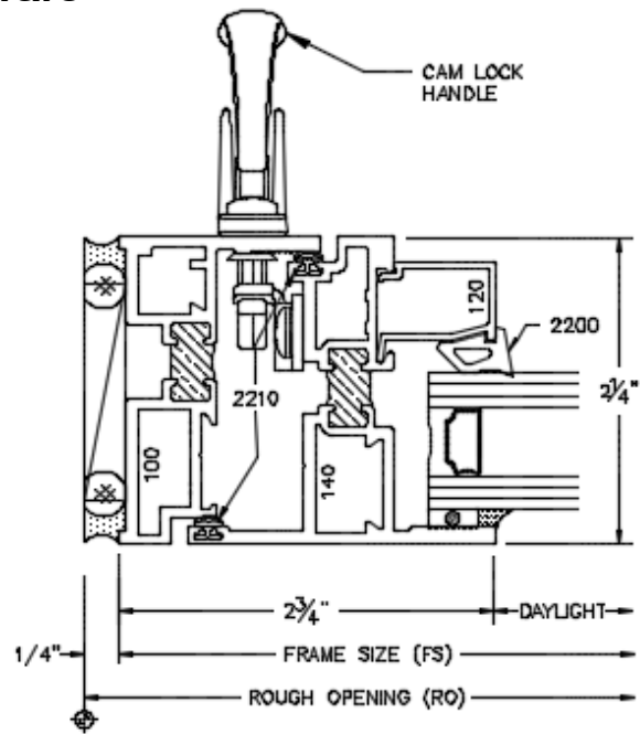
LOCK HANDLE Casement / Awning
