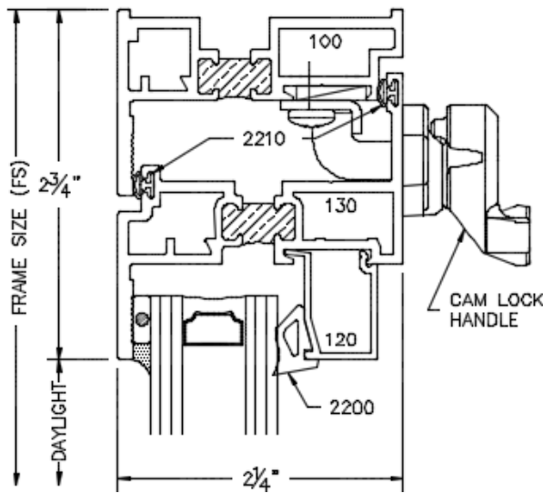
STACK FRAME
