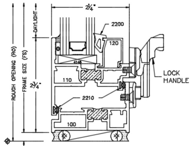
CAM HANDLE Casement / Awning
